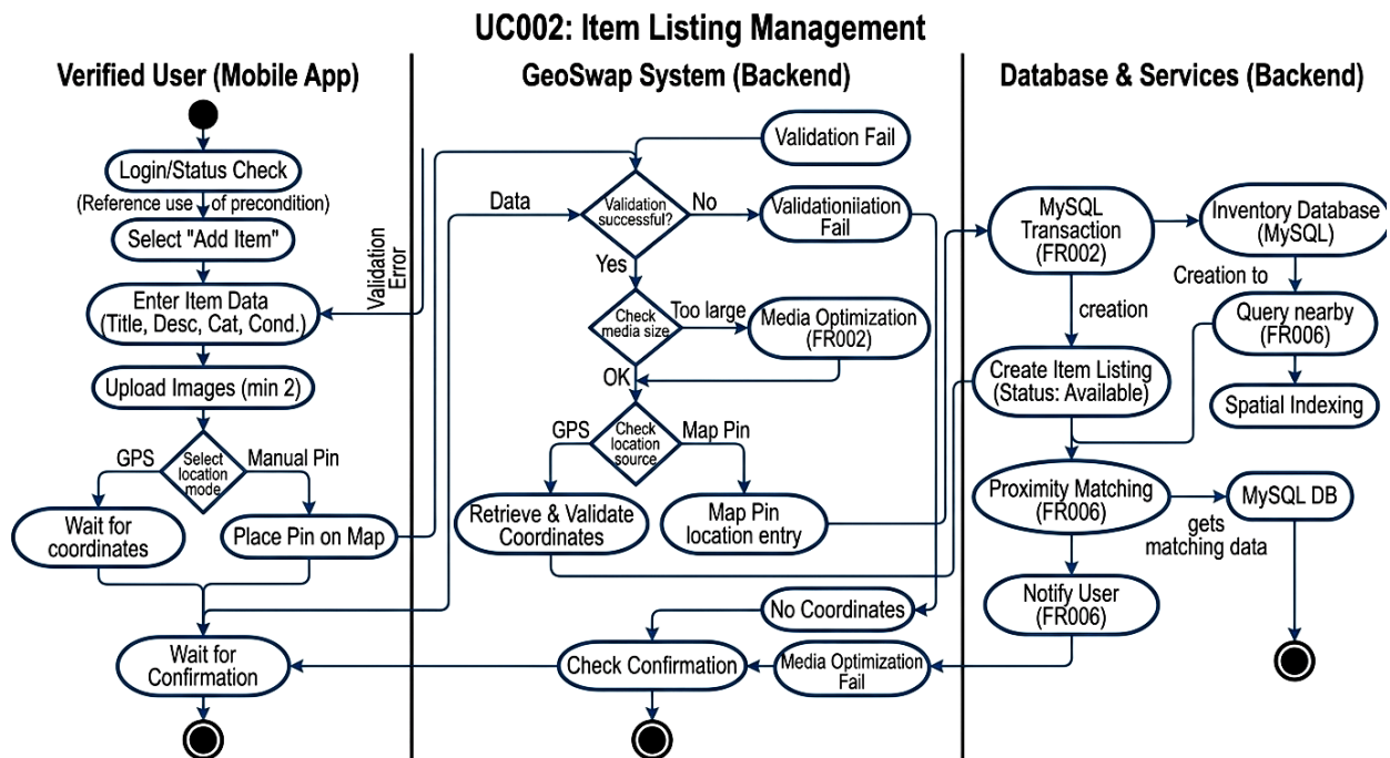
Figure 3: Activity Diagram for Item Listing Management (UC002)
